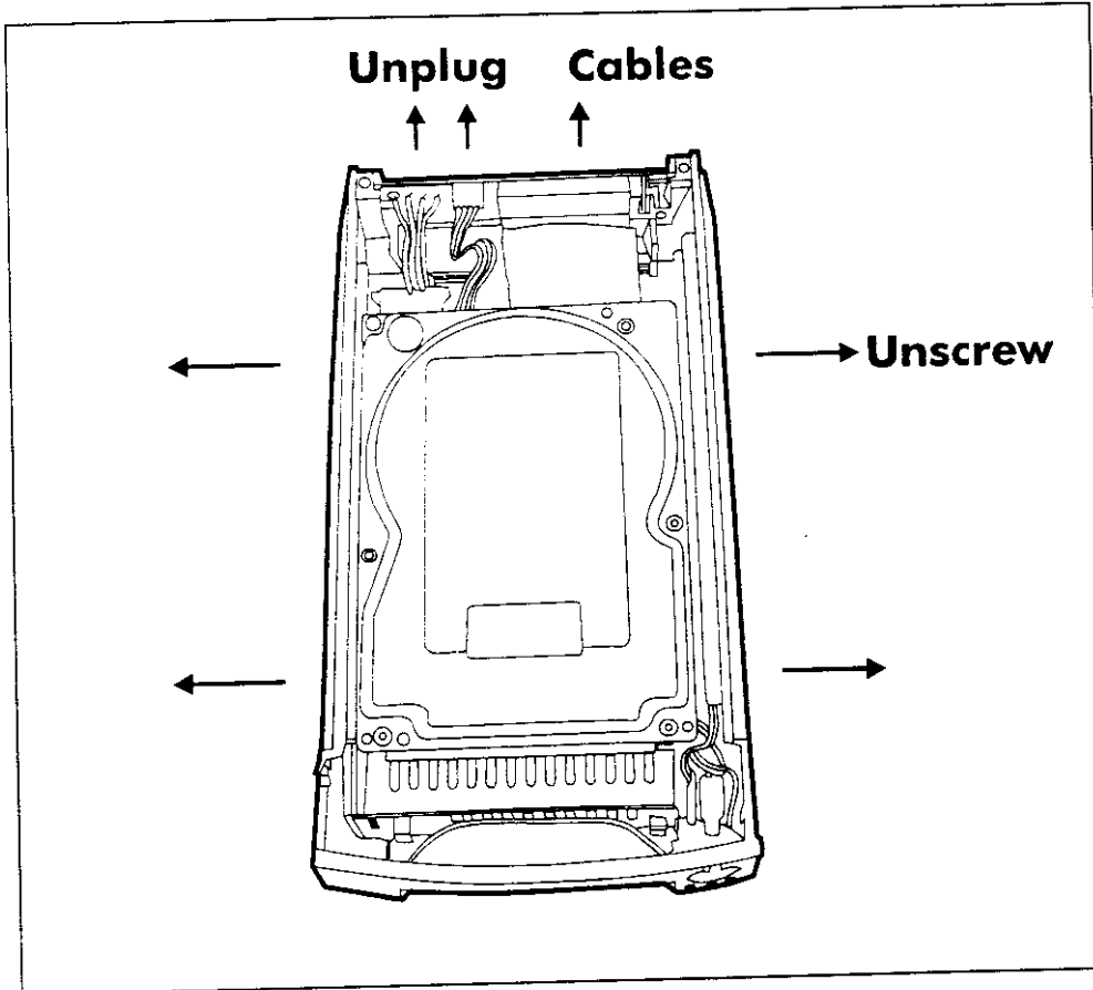
Figure : Swap HDD ( Unplug cables )
