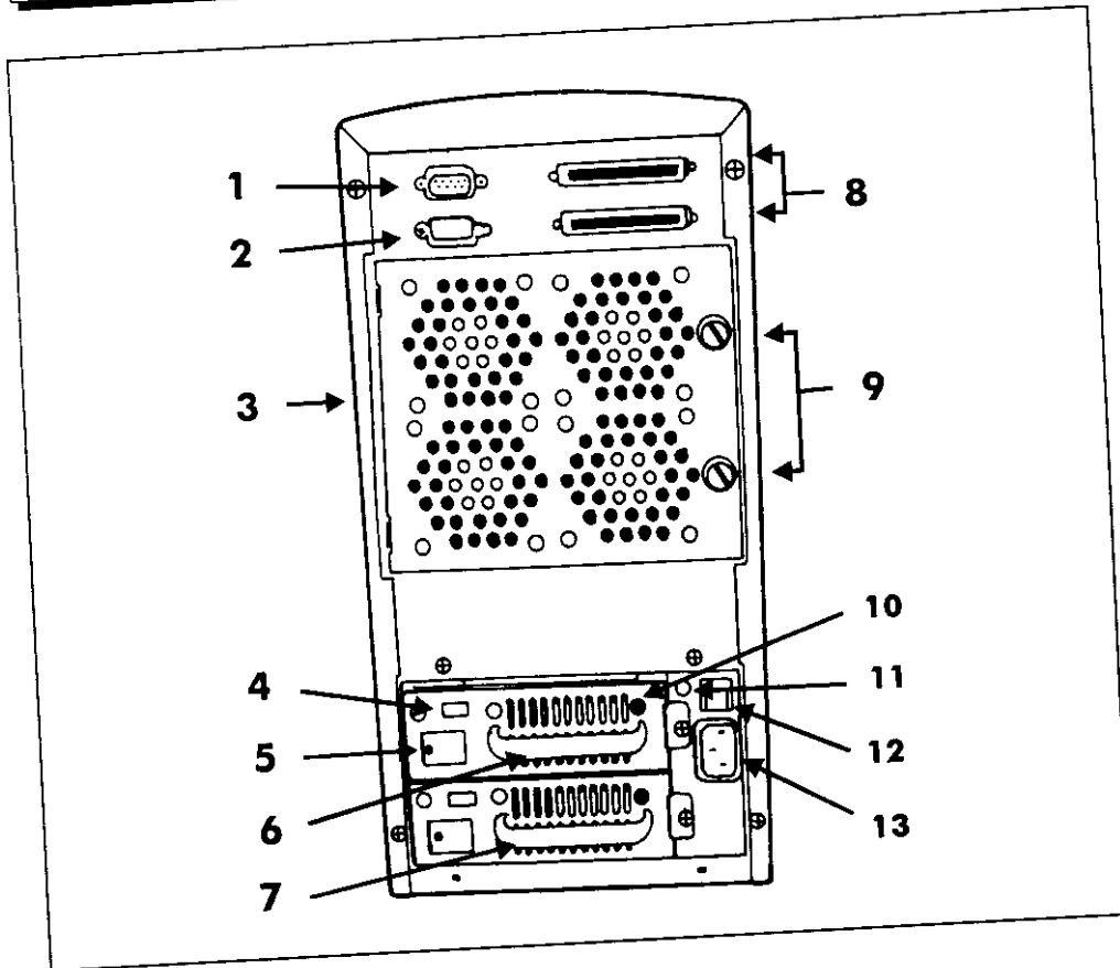
Figure : Rear View
