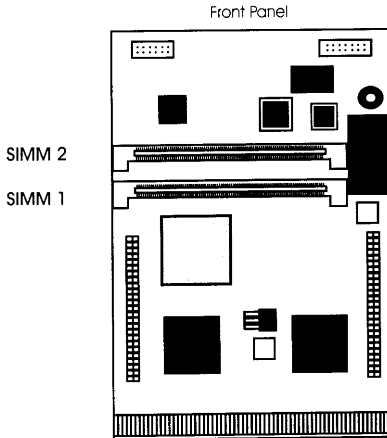
Figure : Controller
