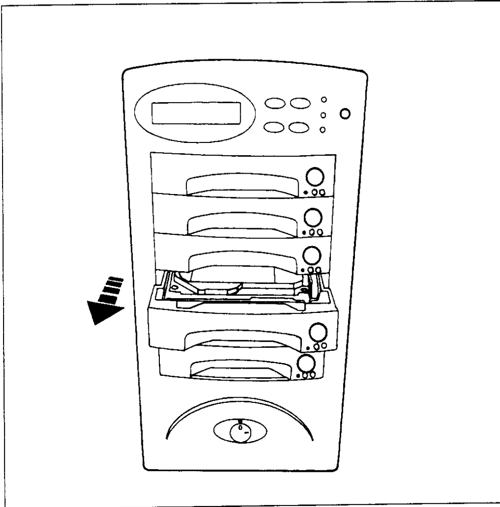
Figure : Swap HDD ( Pull-out )
