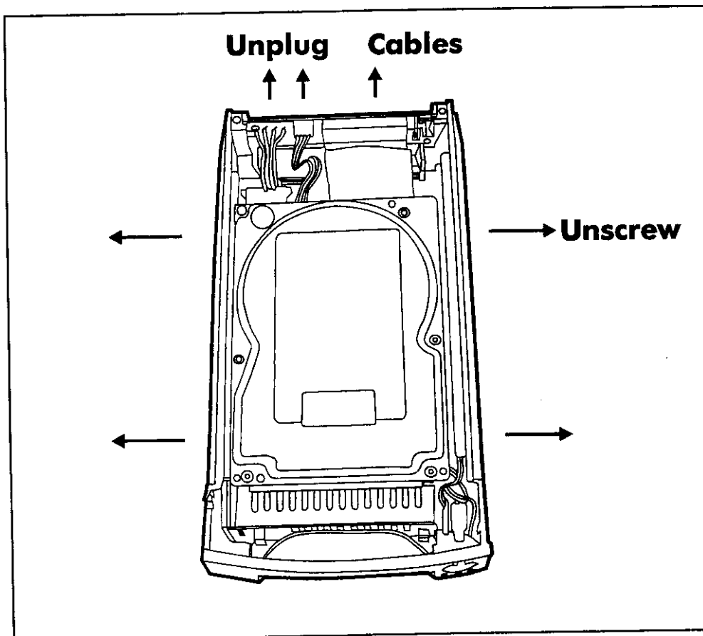
Figure : Swap HDD ( Unplug cables )
