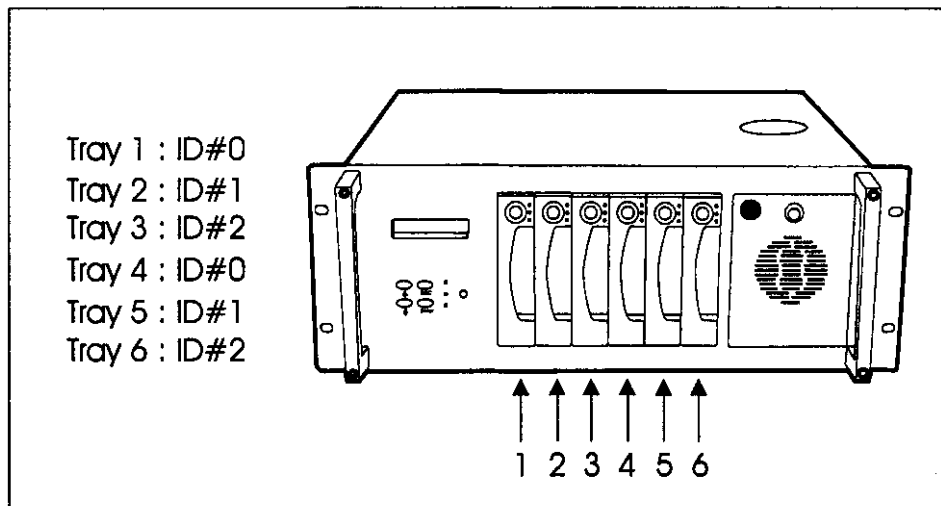
Figure : Manual HDD's SCSI ID setting
