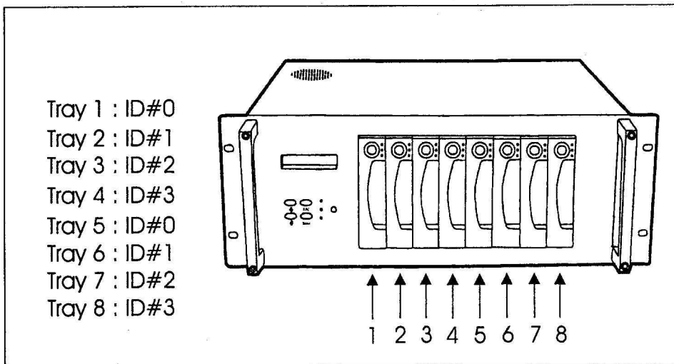
Figure : Manual HDD's SCSI ID setting
