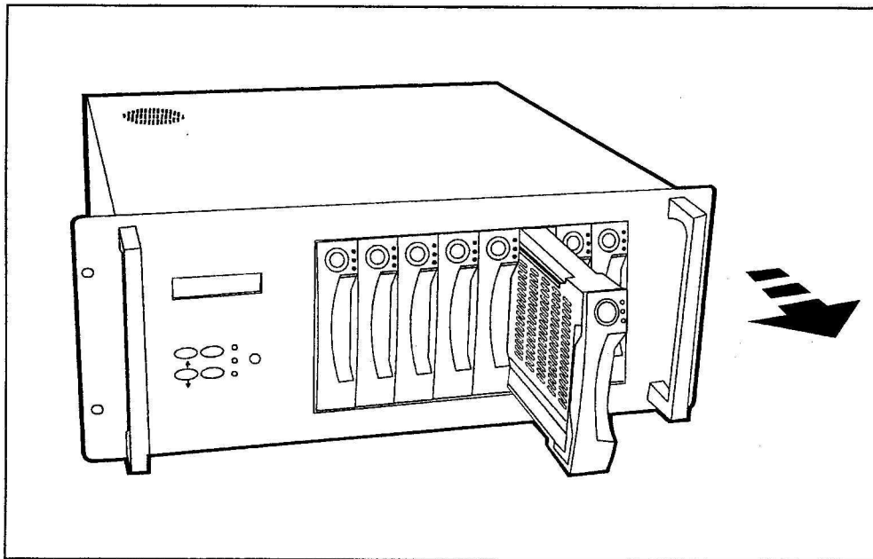
Figure : Installing HDD step 1, 2
