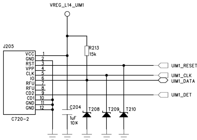
Figure 4.29: UIM card interface circuit
