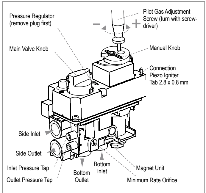
Figure 14: GV60, Connections and Adjustment Options
