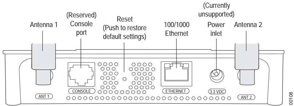
Figure 17: AP200 Connector Panel
