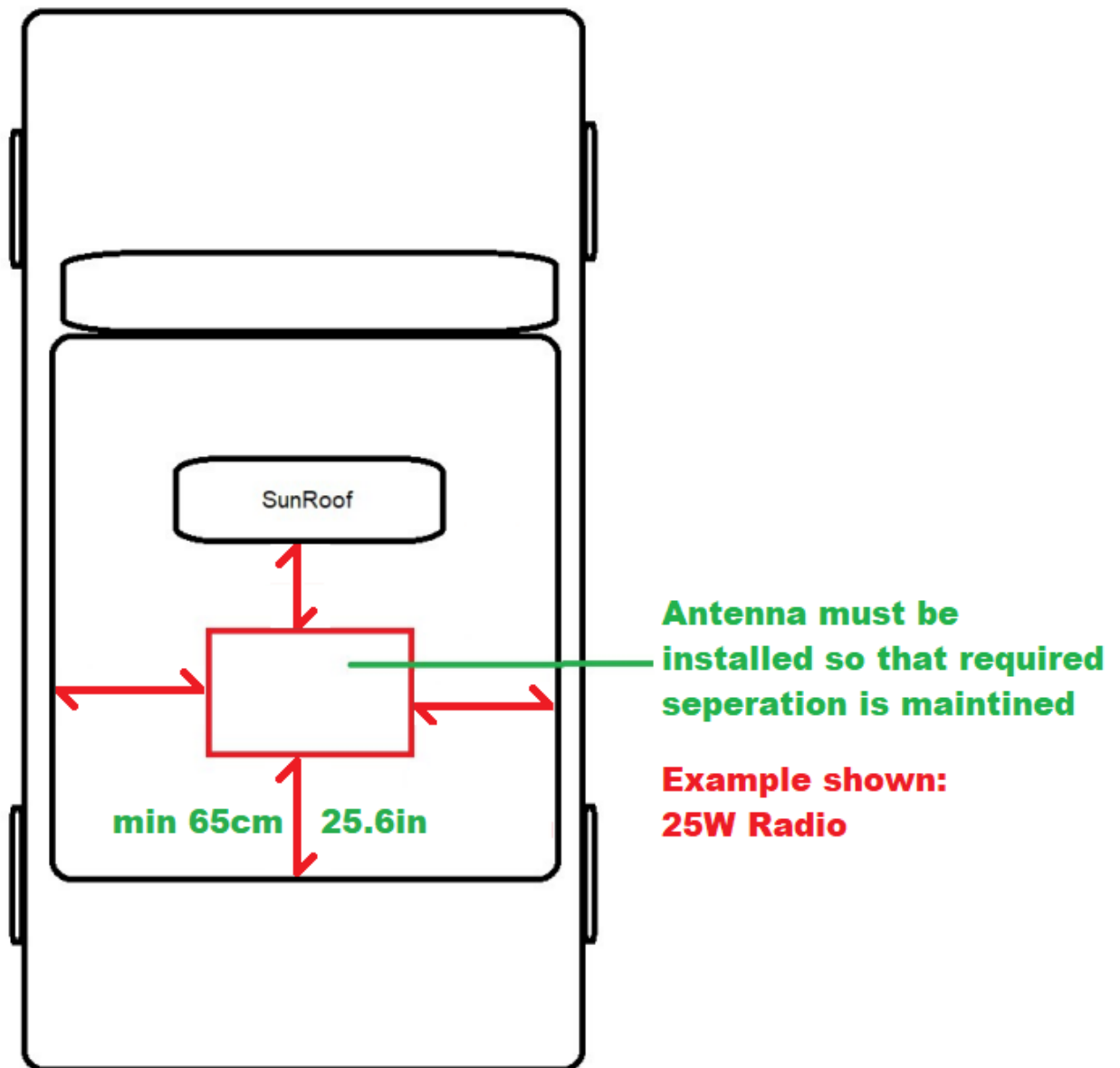
Figure 1: Mounting on vehicle with a sunroof
