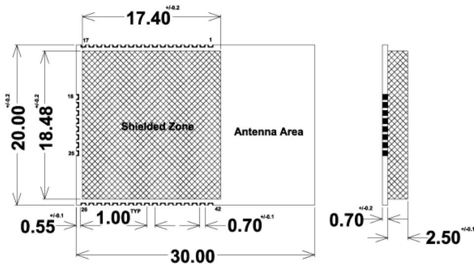
Figure 3-1. ATZB-S1-256-3-0-C Dimensions
