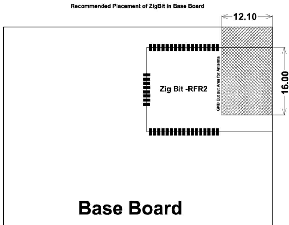
Figure 3-4. ATZB-S1-256-3-0-C Mounting Information
