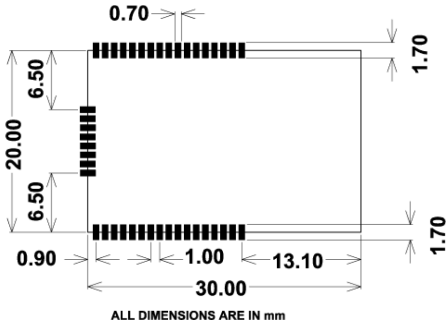
Figure 3-3. ATZB-S1-256-3-0-C Foot Print Dimensions
