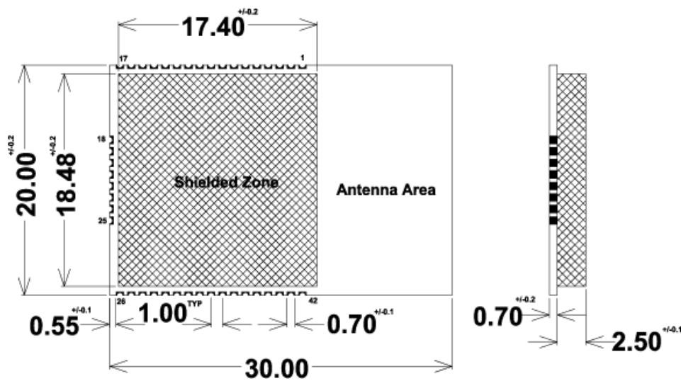
Figure 3-1. ATZB-S1-256-3-0-U Dimensions
