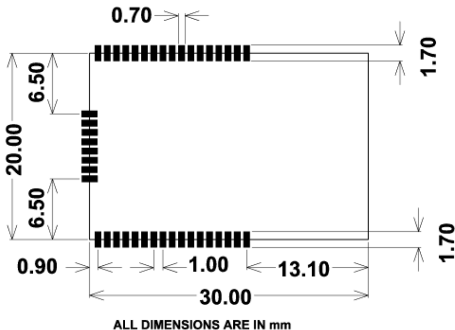
Figure 3-3. ATZB-S1-256-3-0-U Foot Print Dimensions
