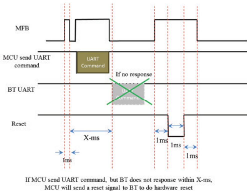
FIGURE 2-6: RESET TIMING SEQUENCE IF MODULE HANGS UP
