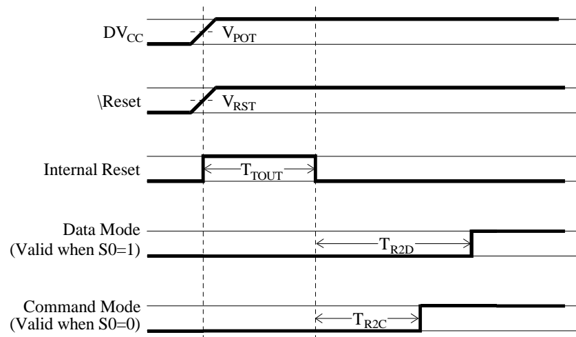
Figure 2. Reset Timing
