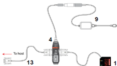
Standalone (5V)
