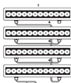
Figure D Hi-Brite Series Illuminators in a daisy chain configuration. See figures A, B, or C for the correct power supply and signal connections for your application.
