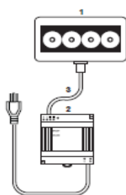
Figure A Hi-Brite Series Illuminator with power supply
