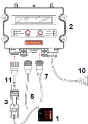
Standalone with MS-Connect 210 (10-28V)
