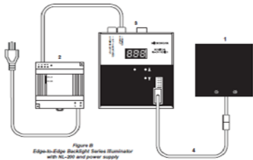
Figure B Edge-to-Edge Backlight Series Illuminator with NL-200 and power supply
