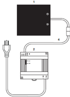
Figure A Edge-to-Edge Backlight Series Illuminator with power supply
