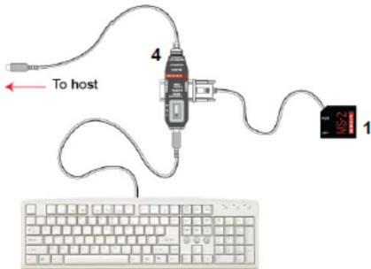
Keyboard Wedge (5V)
