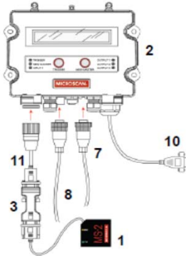
Standalone with MS-Connect 210 (10-28V)
