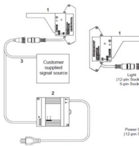
Figure C Pharmalite Illuminator with customer supplied strobe trigger signal source
