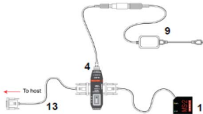
Standalone (5V)
