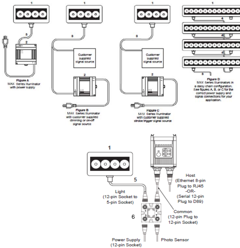
Figure E MAX Series Illuminators with QX-1 Interface Device Note: Figure E is not compatible with daisy chaining. Powering more than one MAX light via the QX-1 will exceed the QX-1's current capability.
