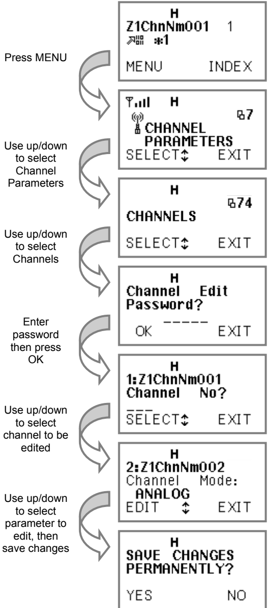
Figure 4.52 – Channel programming
