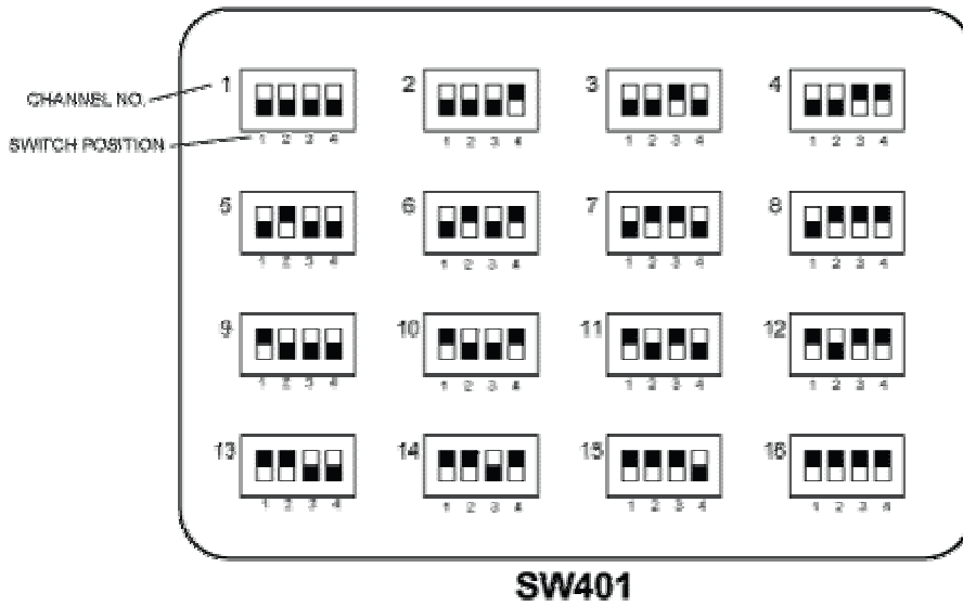
Figure: Setting of channel selector switch for each channel
