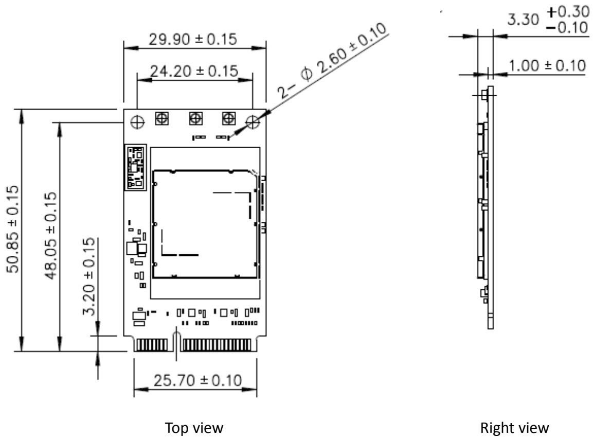
Figure 1. PCBA dimension
