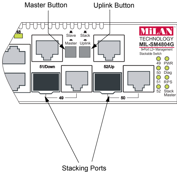
Figure 1-2 Stacking Ports
