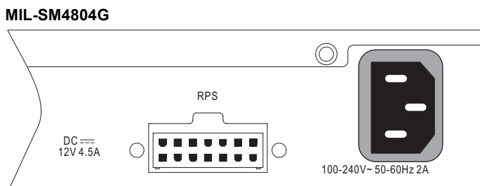
Figure 3-7 Power Receptacles
