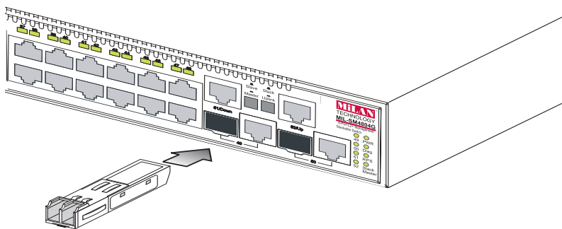
Figure 3-5 Installing an SFP Transceiver into a slot
