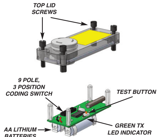
TRANSMITTER ENCLOSURE Shown with Optional Alarm
