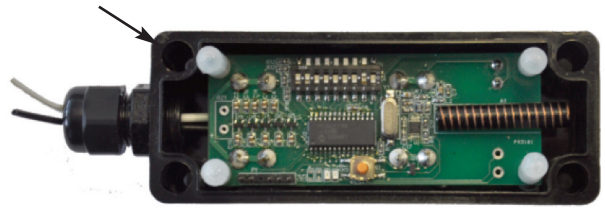
(4) PRE-DRILLED CORNER MOUNTING HOLES
