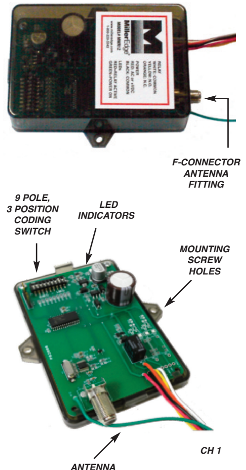
RECEIVER ENCLOSURE
