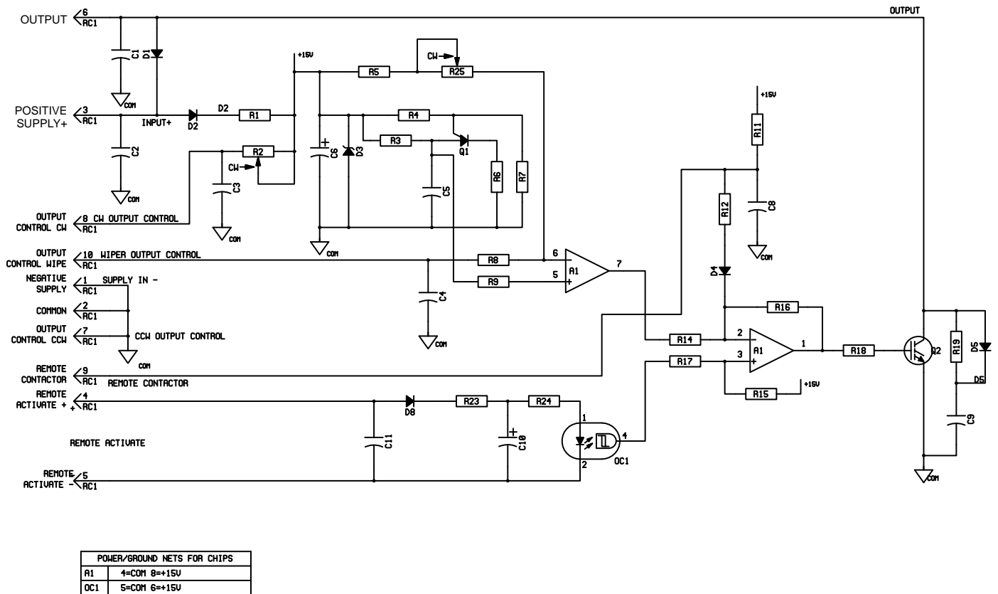
Figure 9-8. Circuit Diagram For Optional Remote Control Board PC3 Effective With Serial No. KA840710 And Following
