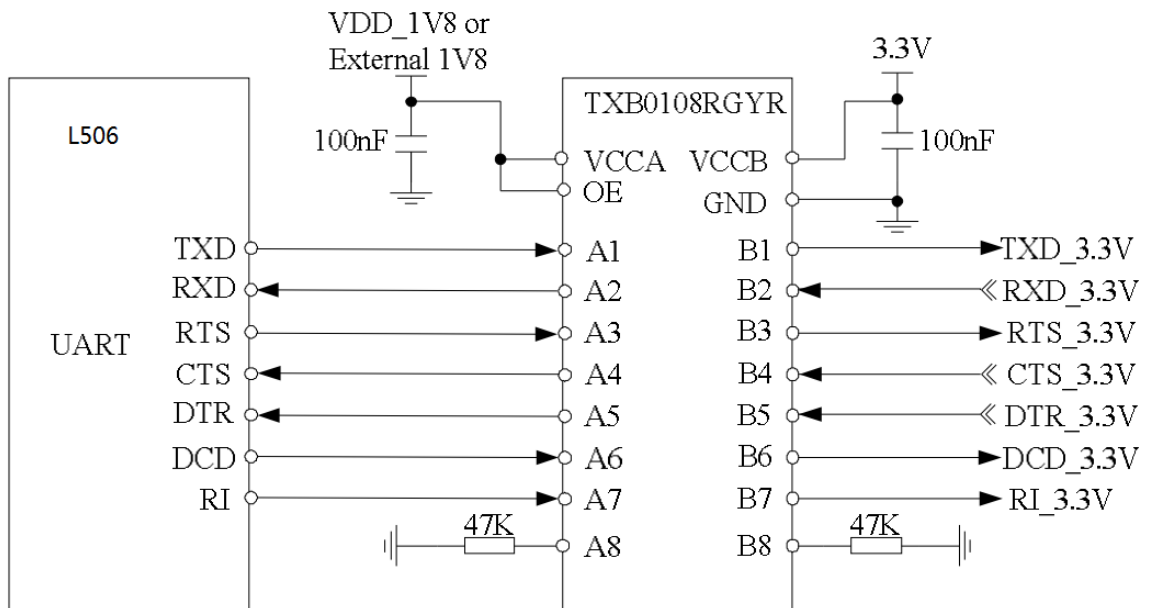
Figure 3-16 Voltage transfer Reference Circuit
