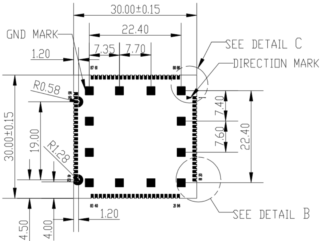
(a) Top Dimensions (Unit mm)
