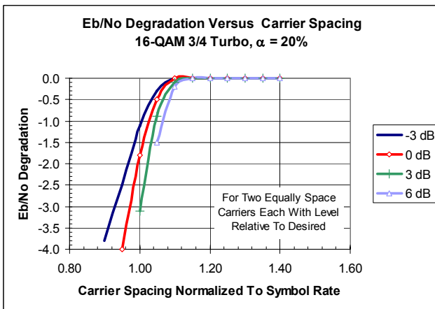
Figure D-4. 16-QAM 3/4 Turbo degradation versus relative carrier spacing (for two adjacent carriers)
