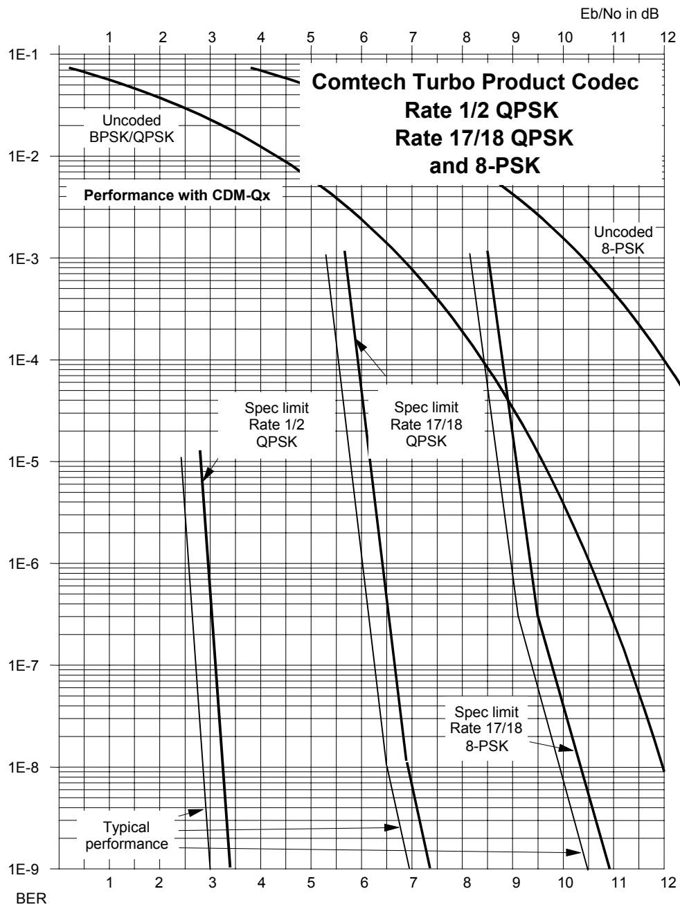
Figure 6-6. Rate 1/2 QPSK, Rate 17/18 QPSK and Rate 17/18 8-PSK
