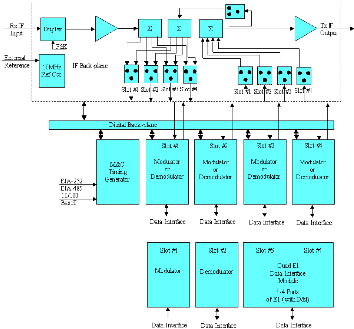
Figure 3-1. Modem Block Diagram
