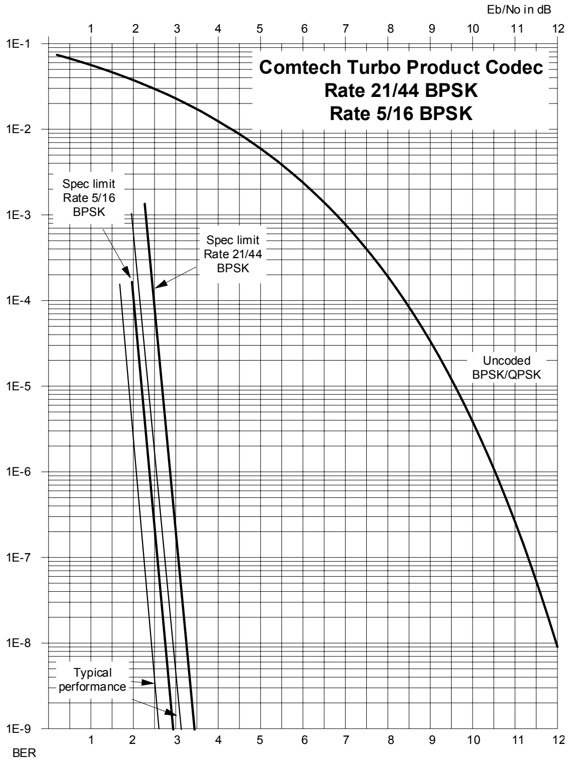
Figure 6-7. Rate 21/44 BPSK and Rate 5/16 BPSK Turbo
