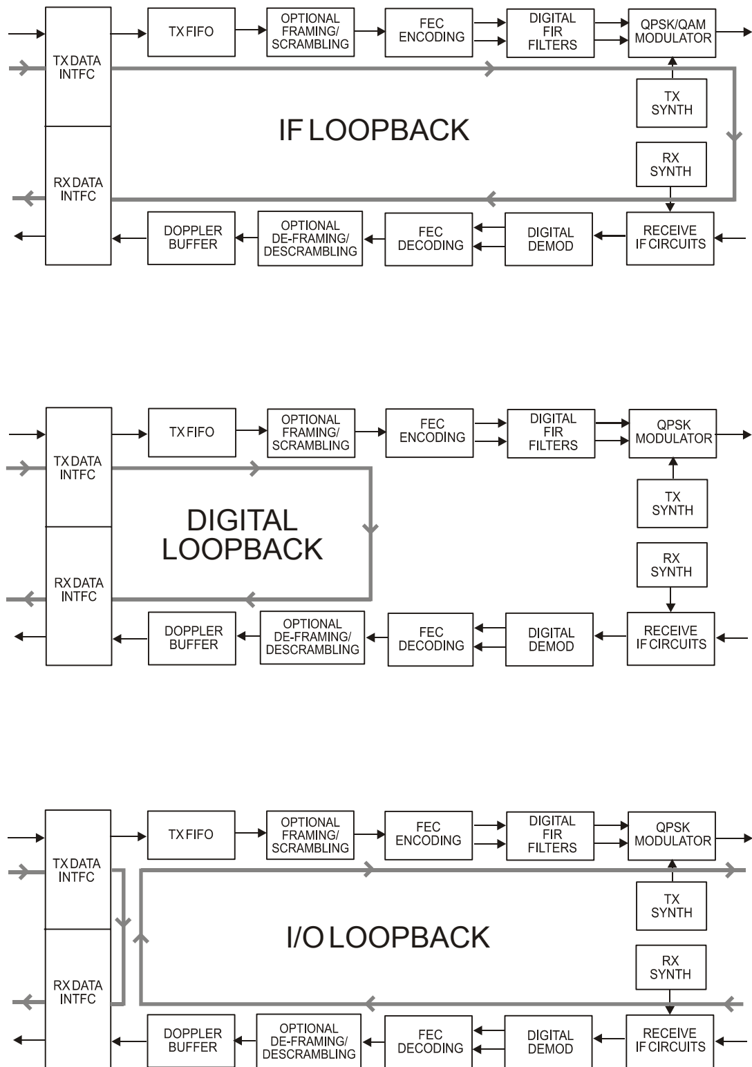
Figure 5-4. Loopback
