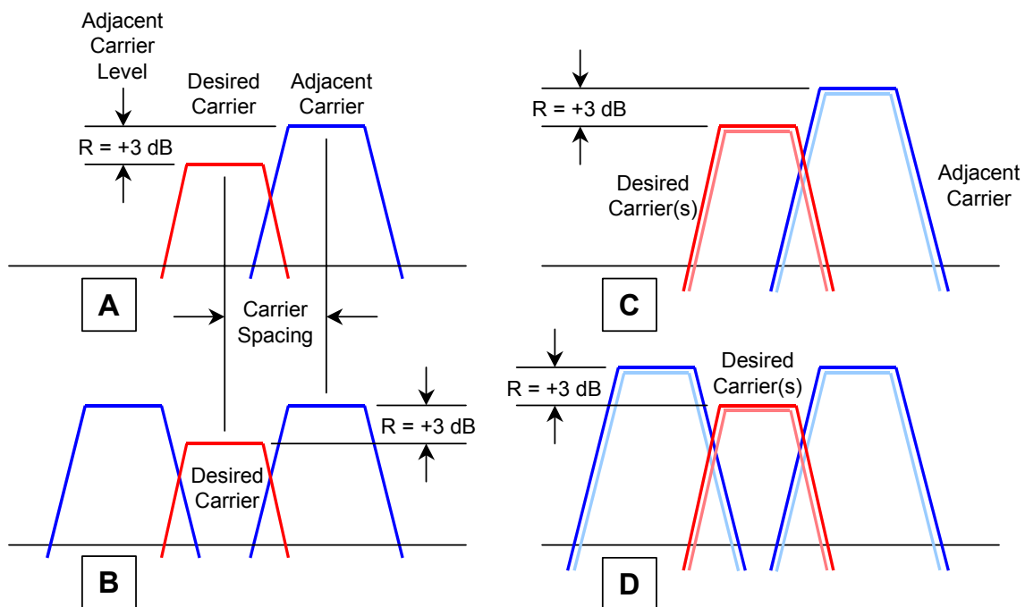
Figure D-5. Adjacent Carrier Cases
