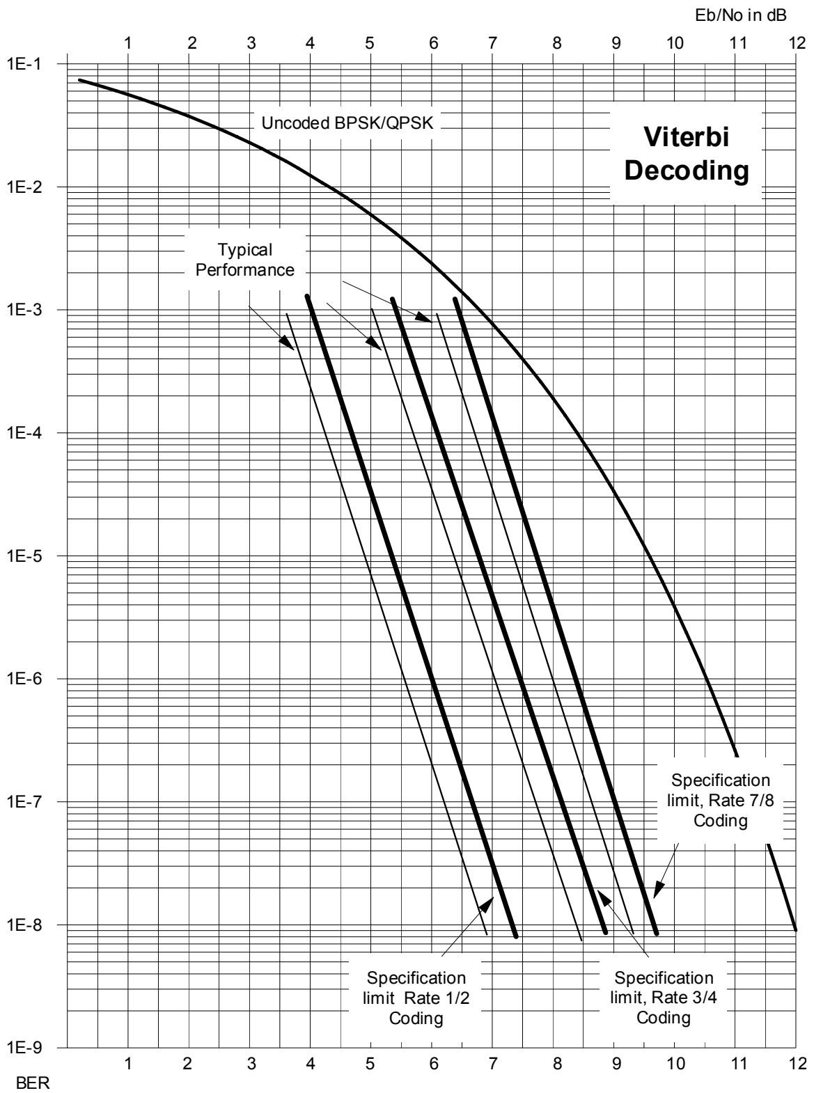
Figure 6-1. Viterbi Decoding
