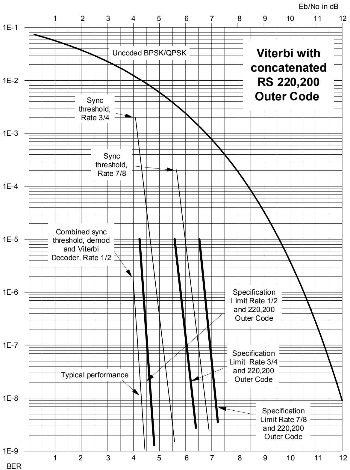
Figure 6-2. Viterbi with concatenated R-S Outer Code
