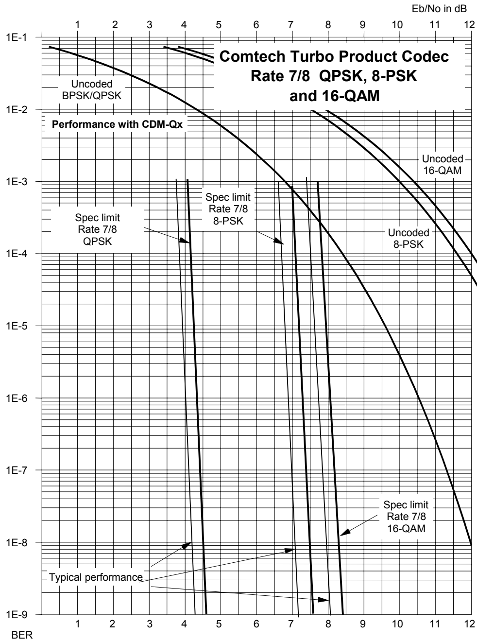
Figure 6-5. Comtech EF Data Turbo Product Codec Rate 7/8 QPSK, 8-PSK and 16-QAM
