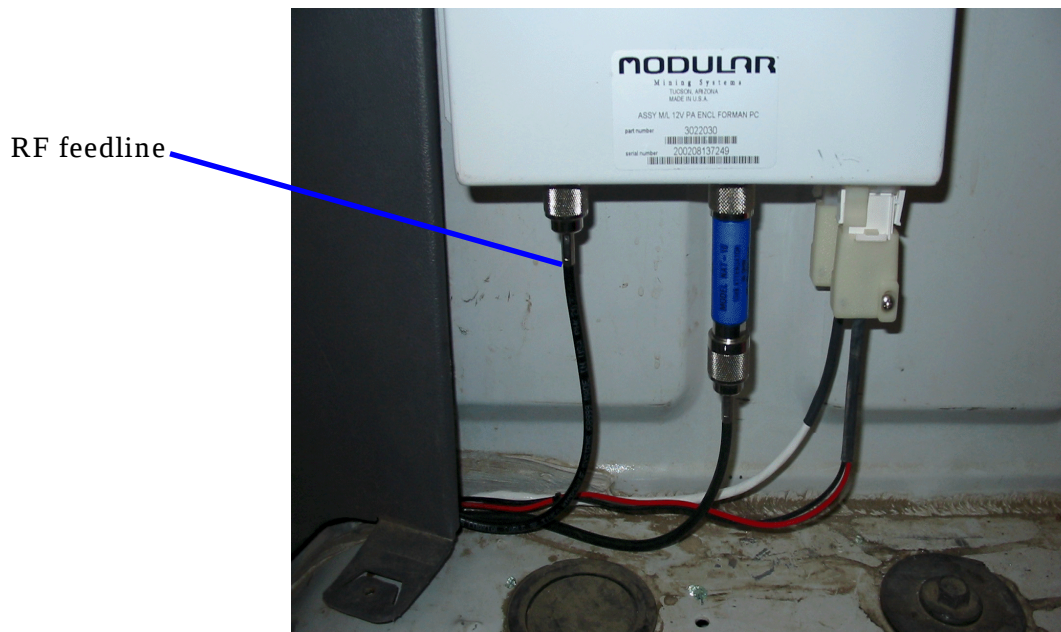
Figure 2.26 RF Feedline Connected
