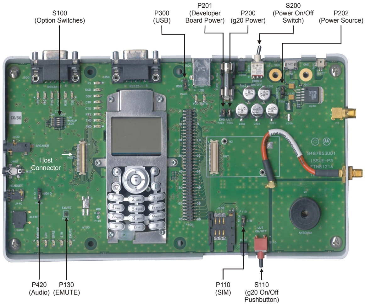
Figure 20. Jumpers and Switches on Developer Board
