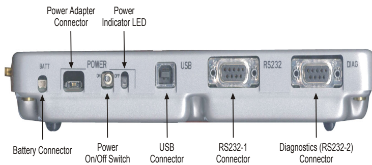
Figure 4. g20 Developer's Kit (rear, with cover)
