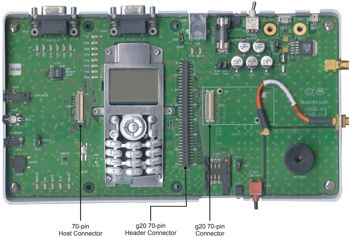
Figure 19. 70-pin Connectors
