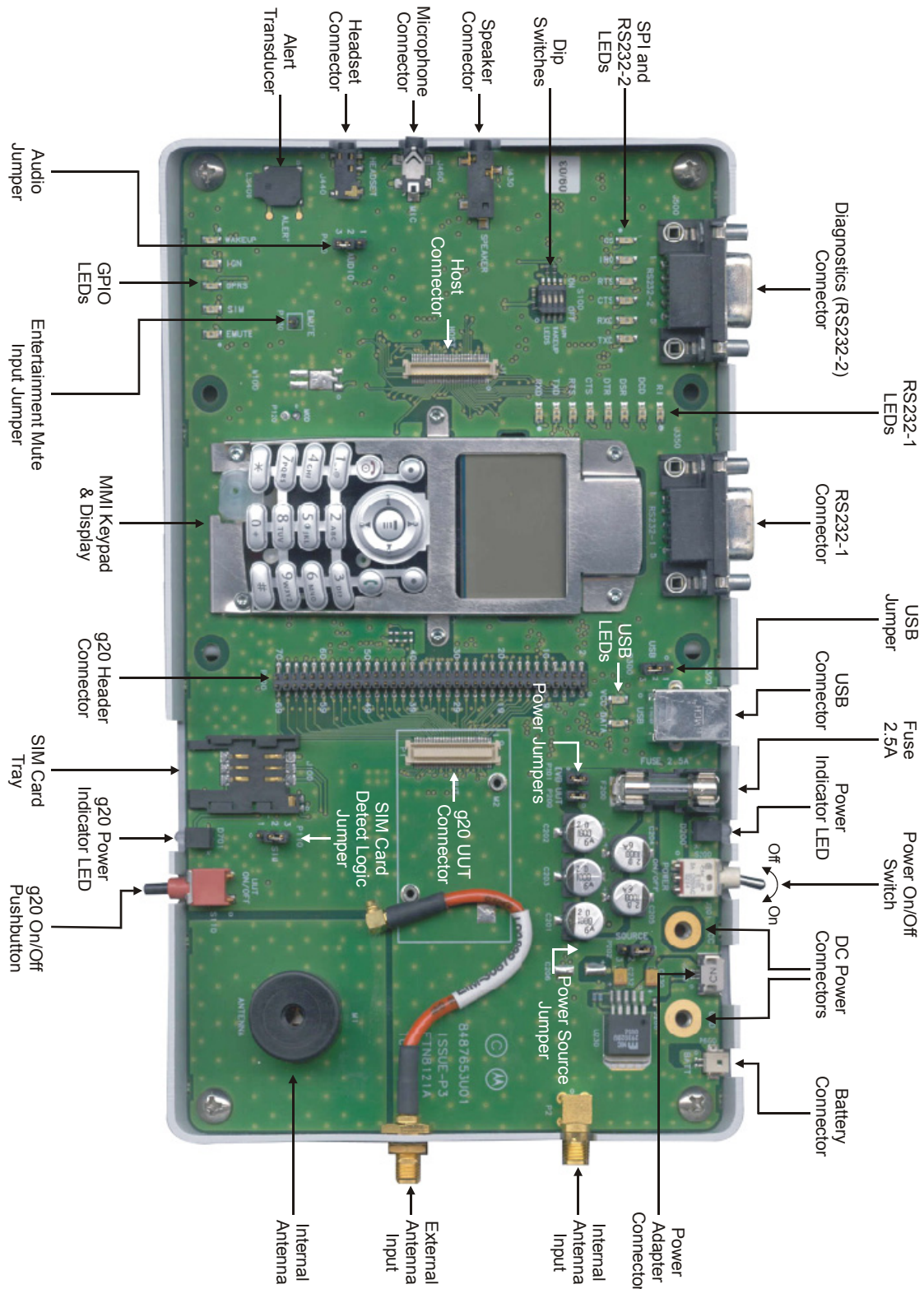
Figure 7. Developer Board Components
