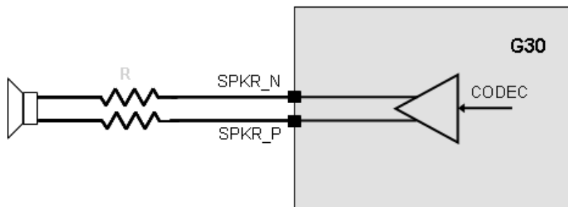
Figure 2-16: Differential Speaker Circuit
