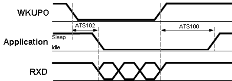
Figure 2-21: WKUPO Operation
