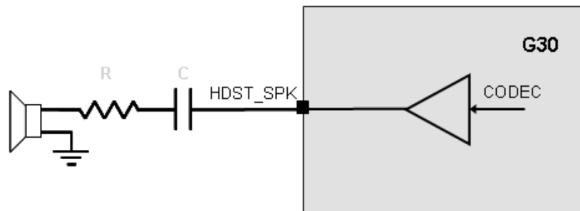
Figure 2-18: Mono Speaker (Headset) Circuit
