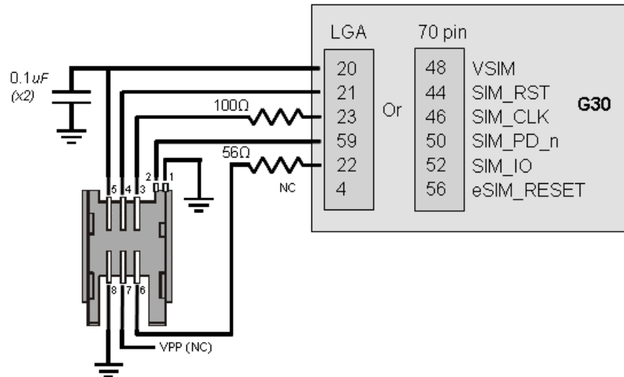
Figure 2-11: G30 External SIM Interface
