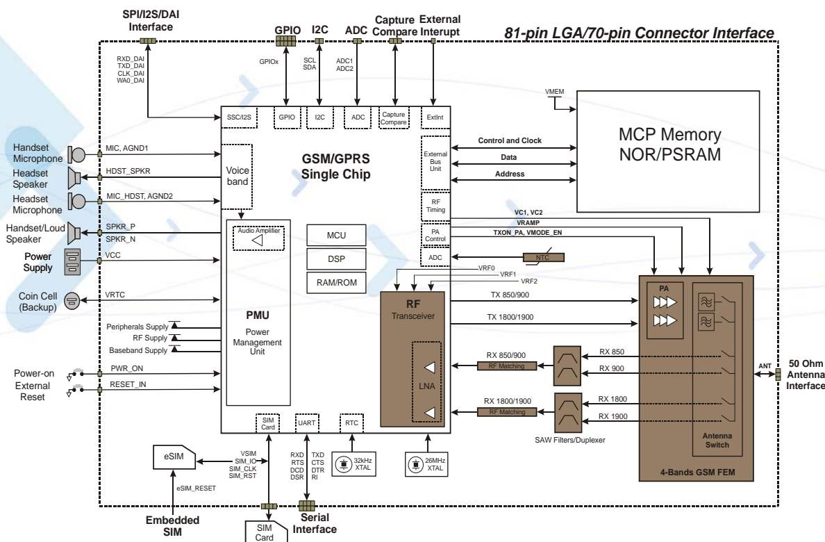
Figure 2-1: G30 Block Diagram
