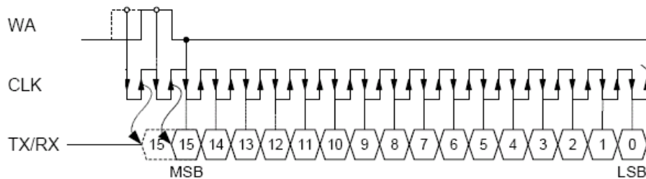
Figure 2-19: Voiceband Mode PCM Bus Coding Format
