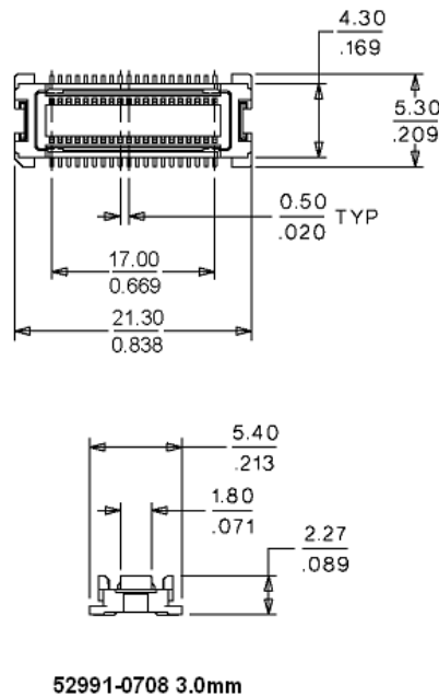
Figure 4-5: Mating Connector Dimensions
