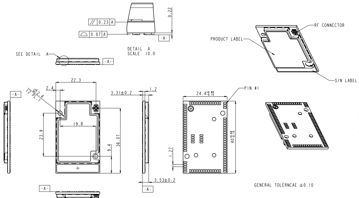
Figure 4-1: G30 Mechanical Characteristics - 81 Pin LGA Interface
