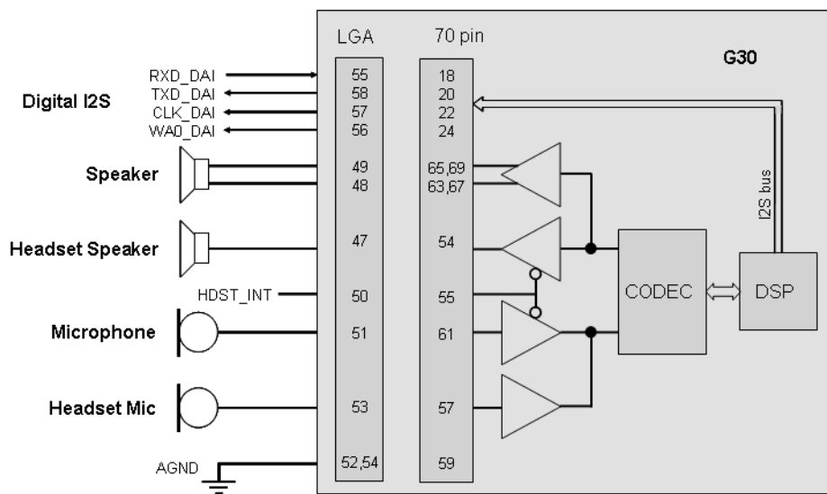
Figure 2-13: Audio Interface Topology
