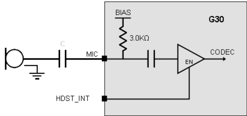
Figure 2-14: Handset Microphone Circuit
