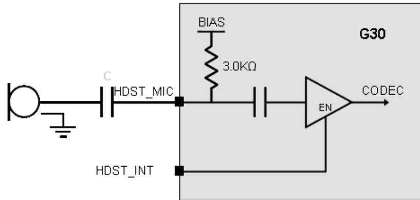
Figure 2-15: Headset Microphone Circuit
