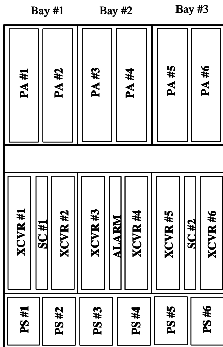
GTR 8000 Expandable Site Sub-system Layout
