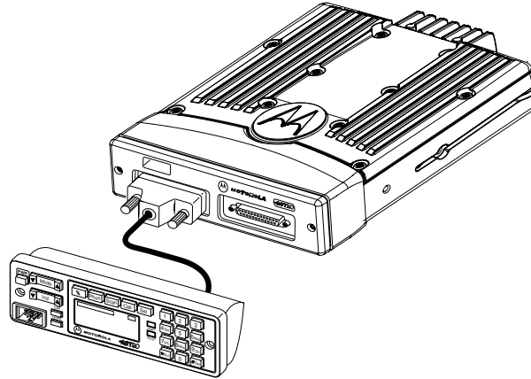
Figure 1-4. Remote Mount Configuration.
