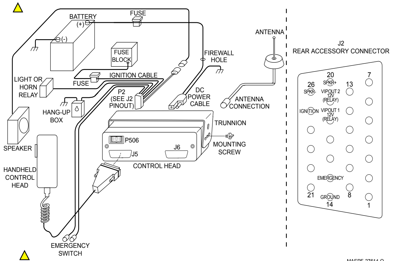
Figure 2-9. Radio Installation (Dash Mount) Using W3 Control Heads
