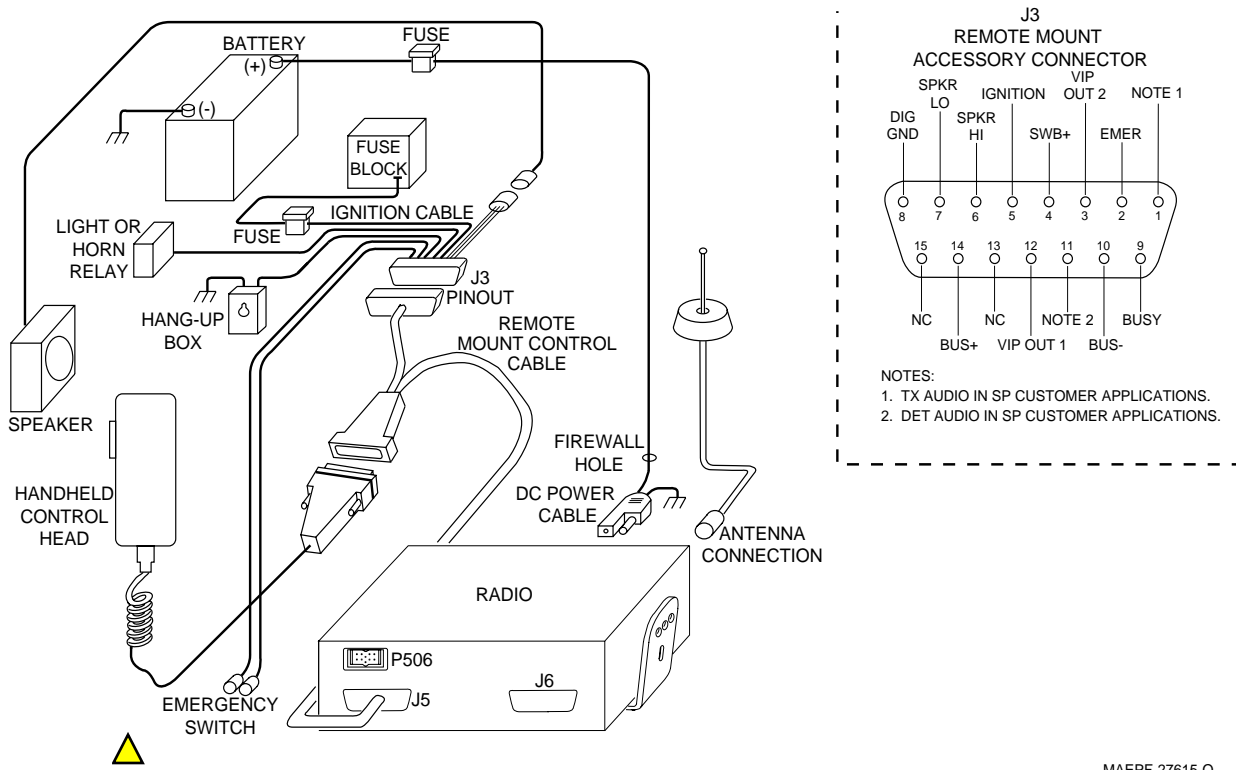
Figure 2-10. Radio Installation (Remote) Using W3 Control Heads
