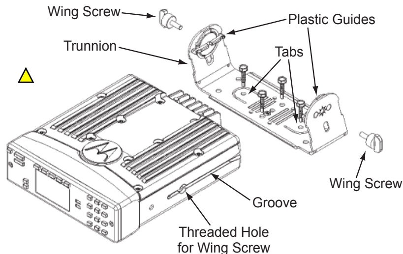
Figure 2-12. Transmission Hump Trunnion Mounting
