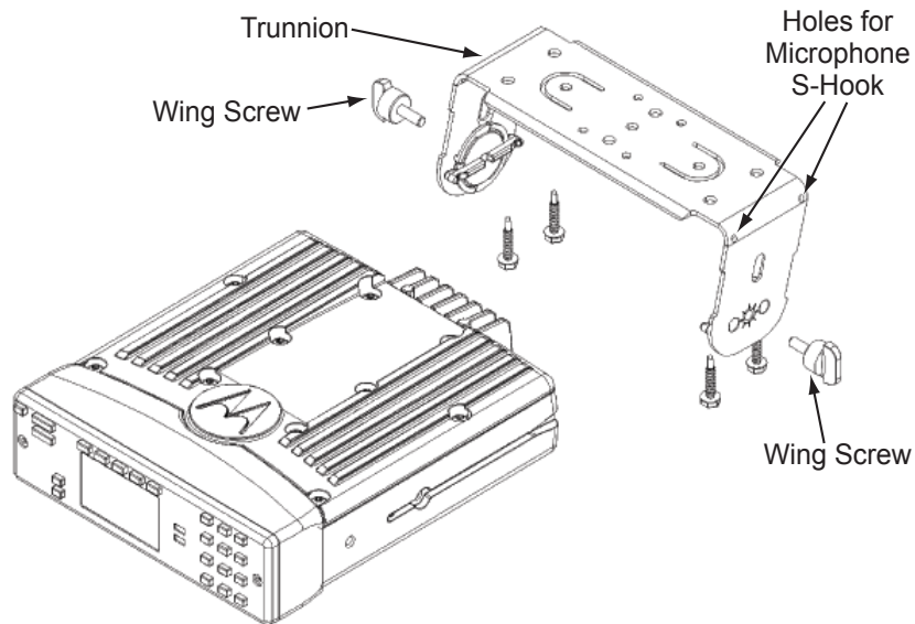
Figure 2-13. Below Dash Trunion Mounting
