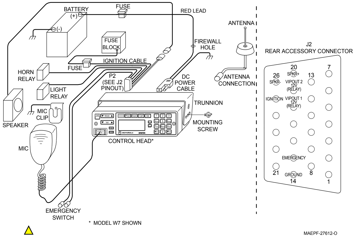
Figure 2-7. Radio Installation (Dash Mount) Using W4, W5, or W7 Control Heads (For complete pin configuration, see Figure 3-9.)
