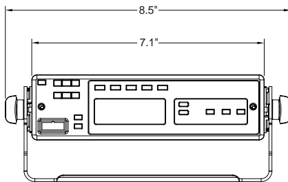
Figure 1-1. Front View of Dash Mount Radio
