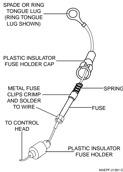
Figure 2-19. Fuseholder Assembly for Orange and Green Control Cables
