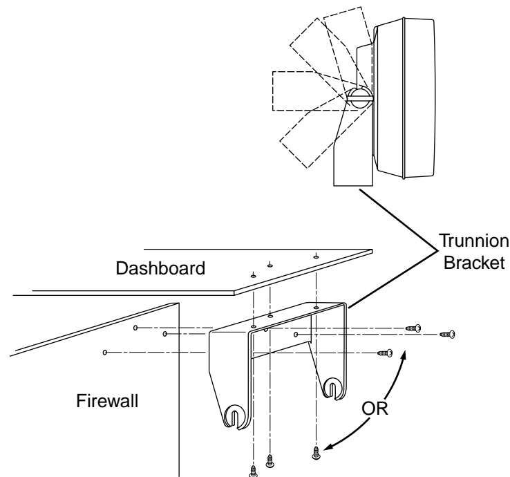
Figure 2-25. Speaker Mounting
