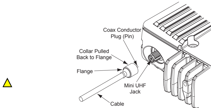
Figure 2-23. Mini-UHF Connector
