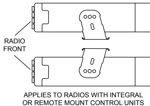
Figure 2-11. Trunnion Orientation
