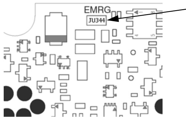
Figure 4-3. Emergency Jumper Removal in Remote Mount
