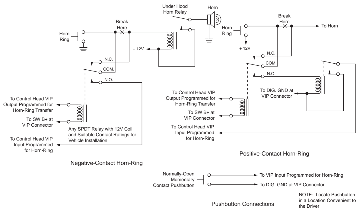
Figure 4-5. Siren/PA Horn-Ring Connections
