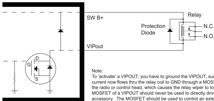
Figure 4-8. Relay Coil
