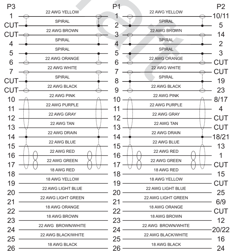
Figure 4-11. Pinout for cable KT000247A01
