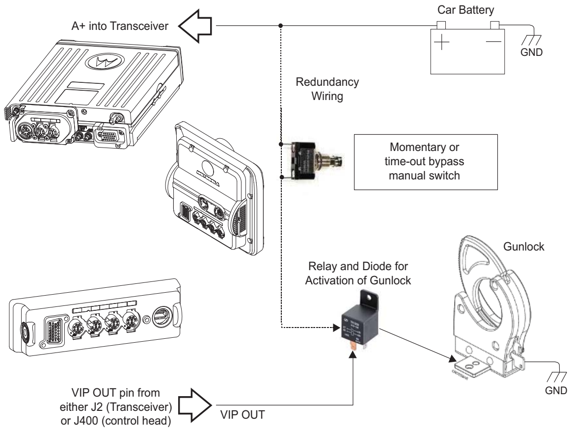
Figure 4-4. Gunlock Switch Redundancy Diagram - Mid Power
