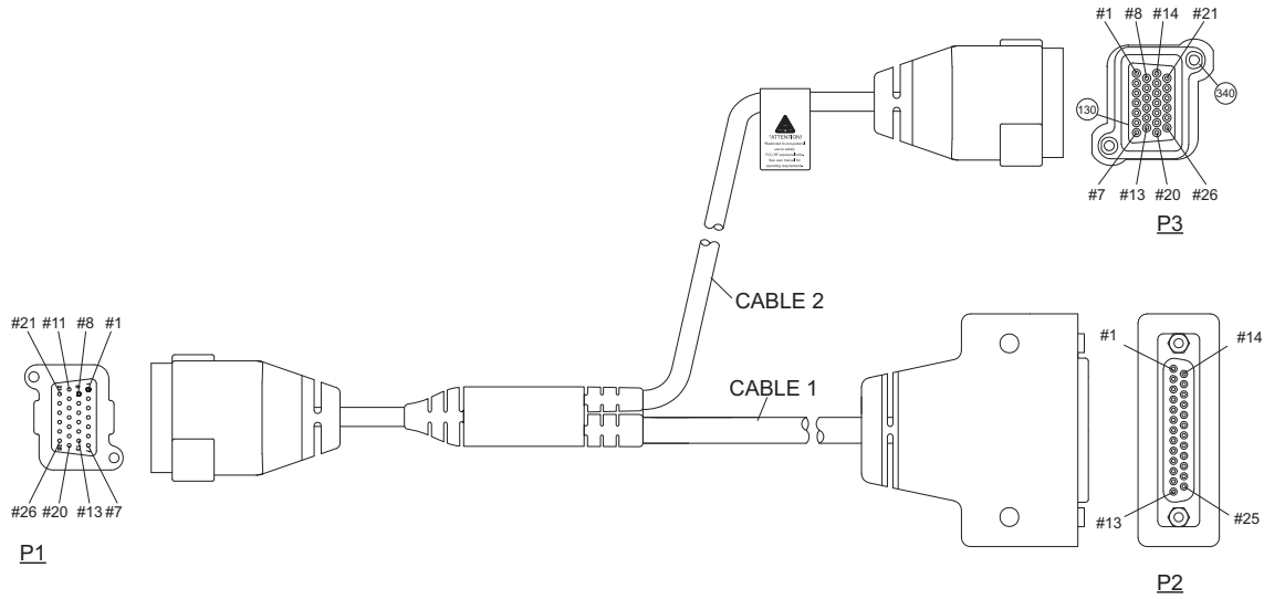
Figure 4-11. J600 Accessory Connector Y-Cable KT000247A01
