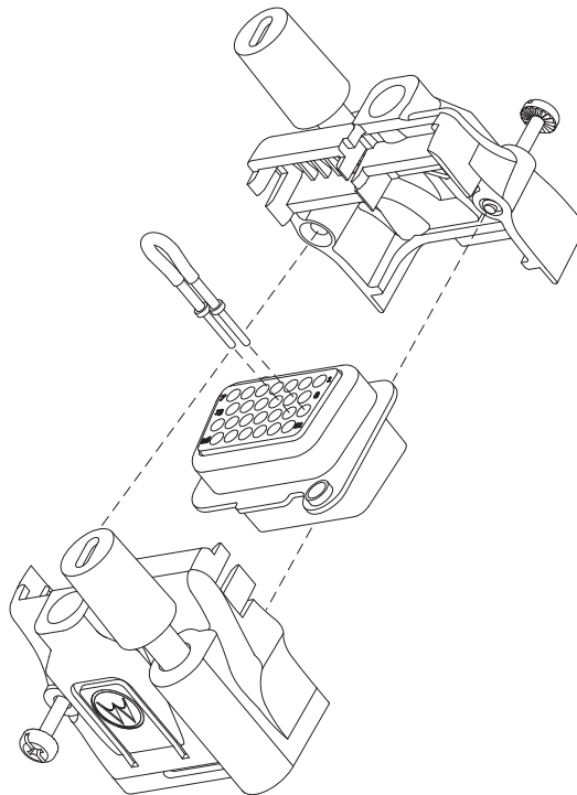
Figure 4-10. Exploded View of Accessory Connector Assembly (HLN6863_)
