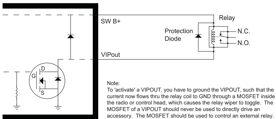
Figure 4-9. Relay Coil
