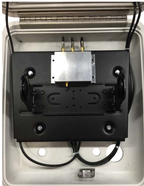
Figure 5-14. Multiplexer and Trunion Mounting
