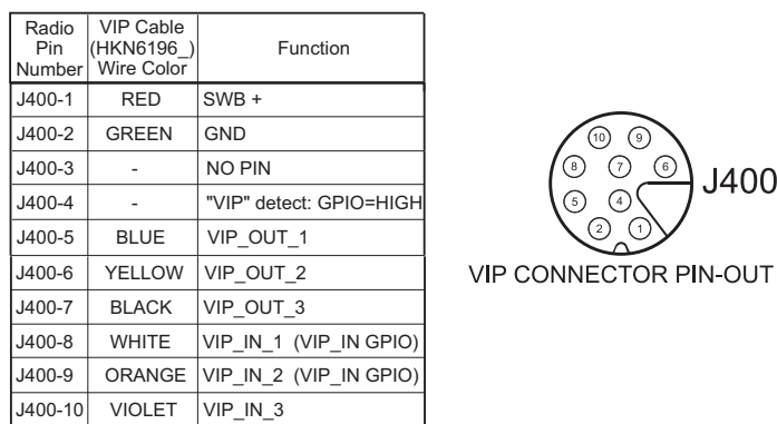
Figure 4-7. Remote Control Head Pinouts
