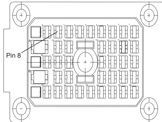
Figure 4-15. Location for Pin 8
