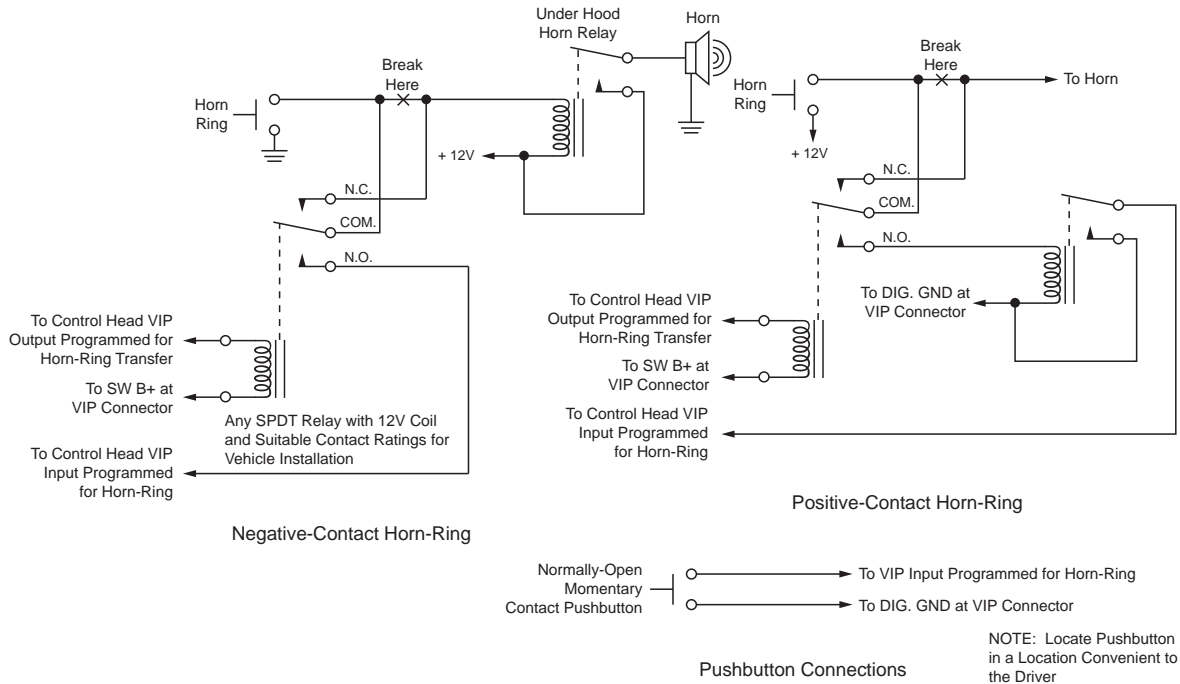
Figure 4-6. Siren/PA Horn-Ring Connections
