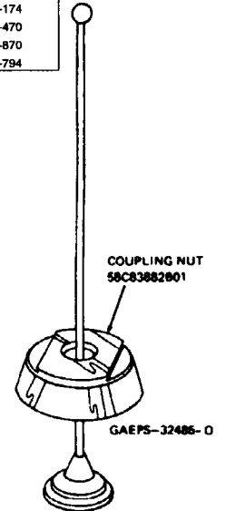
Figure 1. Whip Parts Identification
