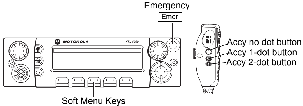
Figure 1: Programmable Buttons on the Keypad Microphone
