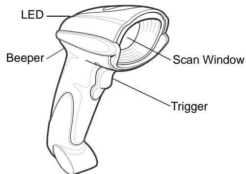
Figure 1-1 Symbol DS6708 Digital Scanner
