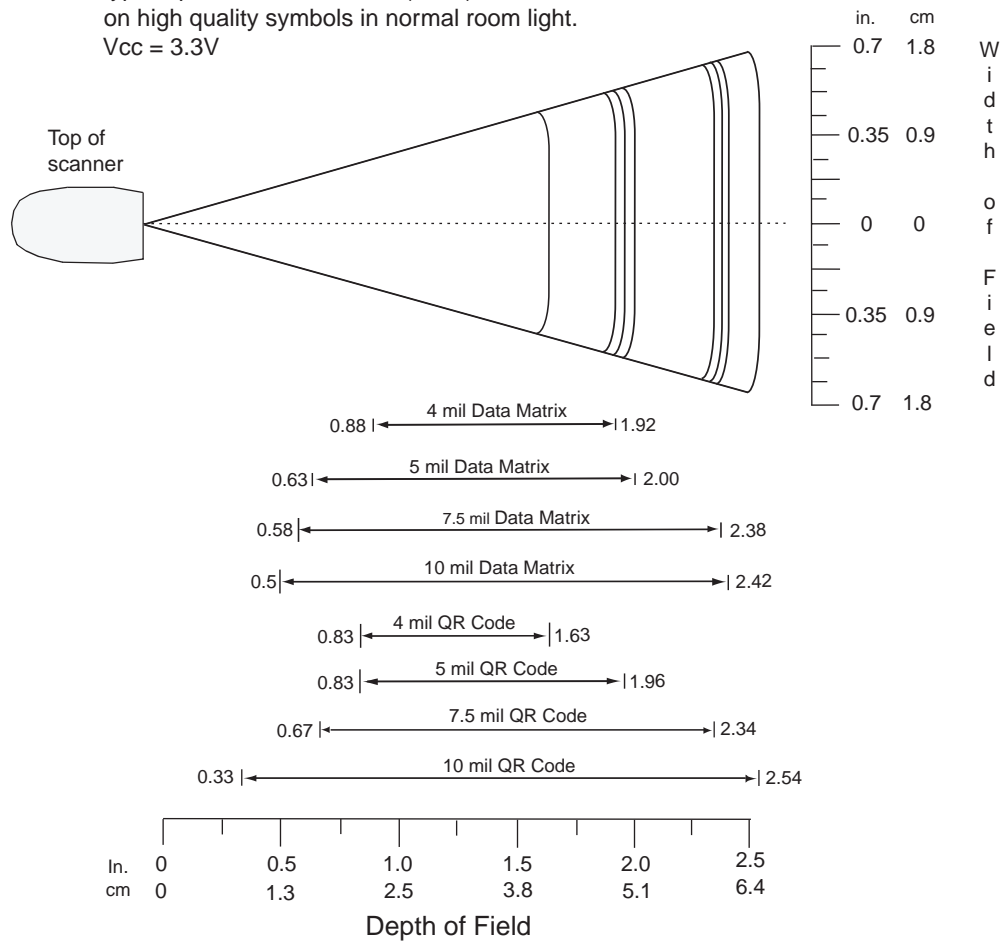
Figure 2-11 DS3478-HD/DPM Near Focus Decode Zone - 2D Codes
