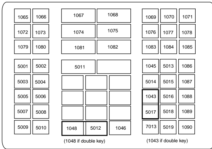
Figure 6-5 NCR 7052 58-KEY
