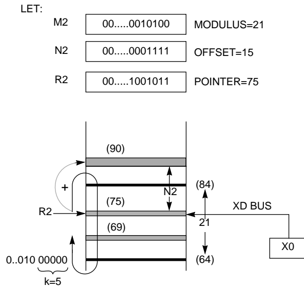
Figure 4-13 Modulo Modifier Example
