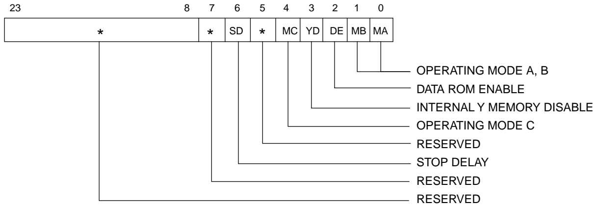
Figure 5-6 OMR Format
