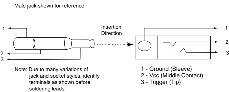
Figure 2-7 Trigger Jack Connector Pins
