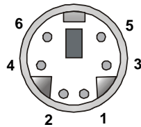
PS/2 Mouse / Keyboard (6-pin Female)
