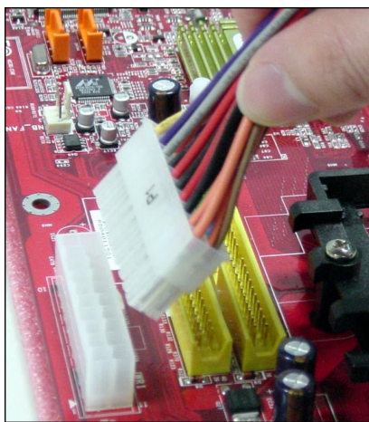
Figure 2: Unplug the ATX1 power connector
