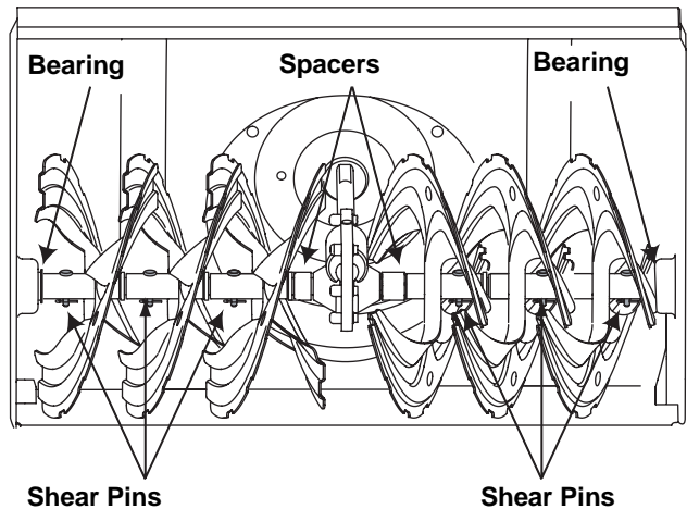
Figure 21- 30" Auger Shown
