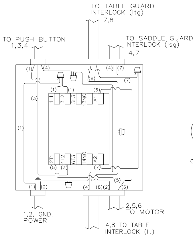
(SK 737W2 Relay Wiring)
