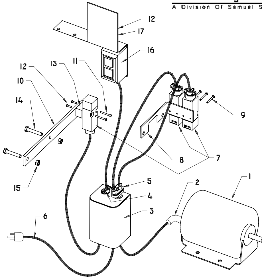
(SK 737W2 Exploded)
