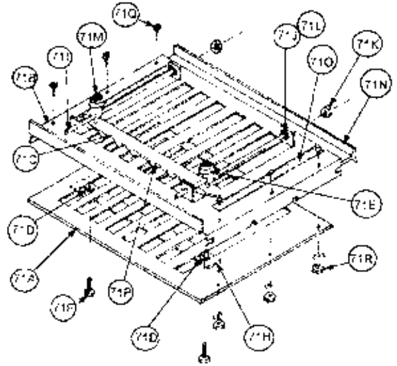
Parts Diagram #2
