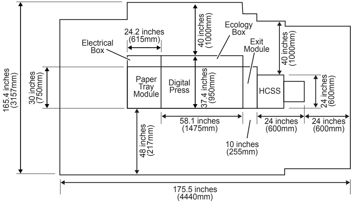
Figure 6-8. Printer with High Capacity Stacker Stapler (HCSS)
