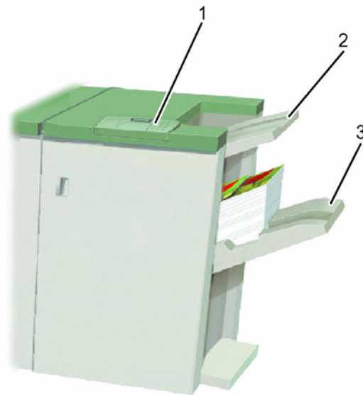
Figure 3-15. High-capacity stacker stapler (HCSS)
