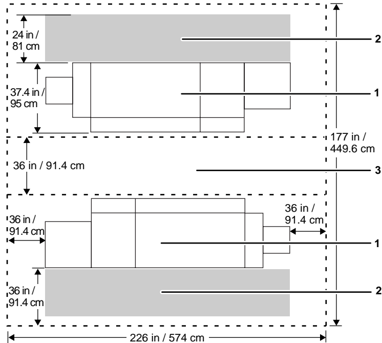
Figure 6-10. Back-to-back shared service area space
