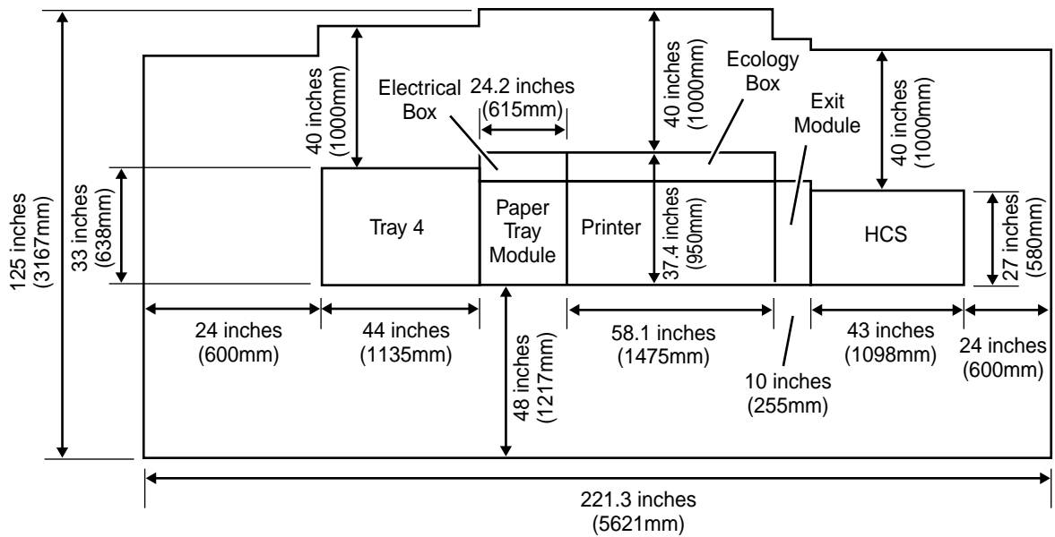
Figure 6-7. Printer with Tray 4 and High Capacity Stacker (HCS)
