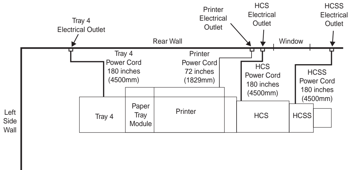
Figure 6-3. Outlet placement for 2060 NPS/IPS
