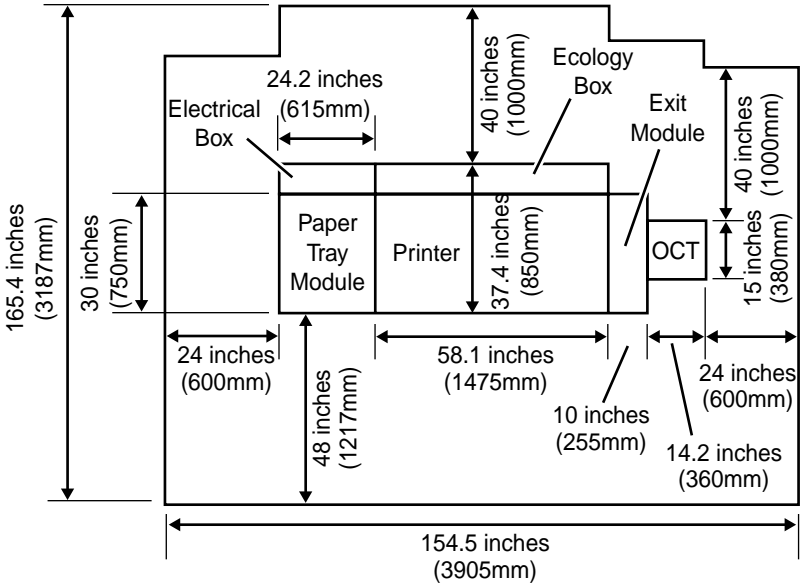
Figure 6-4. Printer
