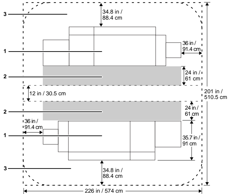
Figure 6-11. Face-to-face shared service area space
