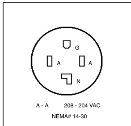
Figure 6-1. DocuColor 2060 NPS/IPS outlet
