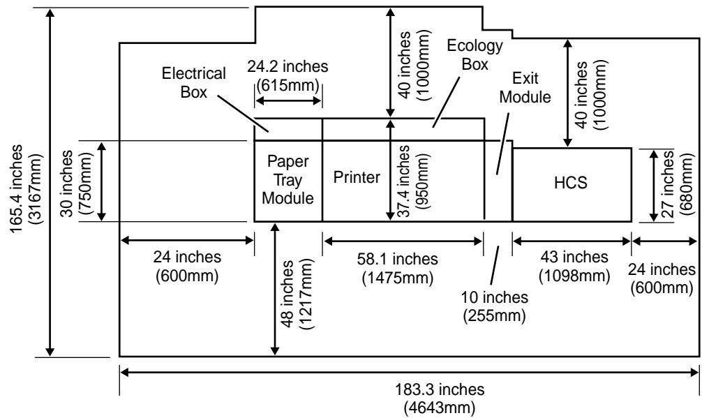
Figure 6-6. Printer with High Capacity Stacker (HCS)
