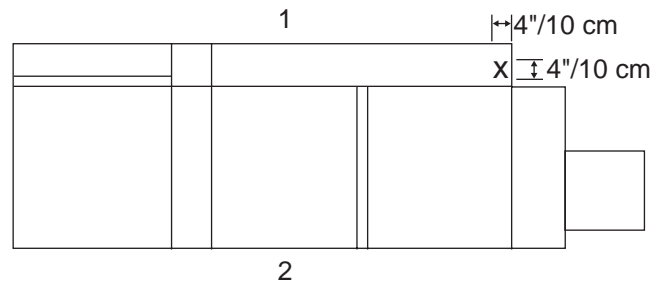
Figure 7-1. Cable enter/exit location (top view)
