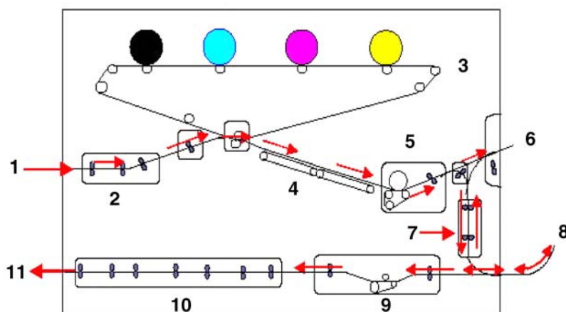
Figure 3-10. Printer paper path
