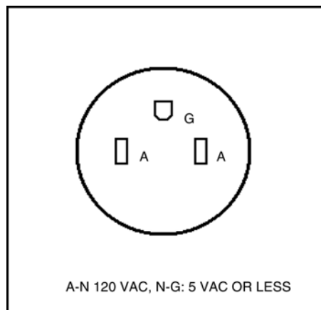
Figure 6-2. Accessories outlet
