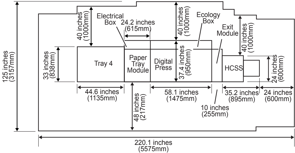
Figure 6-9. Printer with Tray 4 and High Capacity Stacker Stapler
