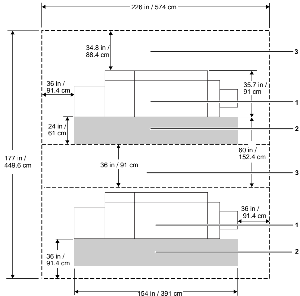
Figure 6-12. Face-to-back shared service area space
