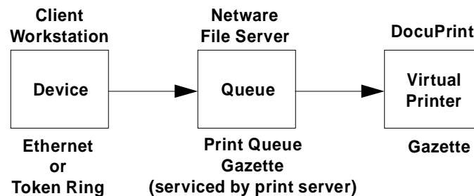
Figure D-3. DocuColor 2060 NPS/IPS configured as a PSERVER
