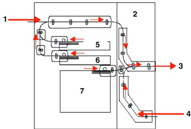
Figure 3-7. Paper Path
