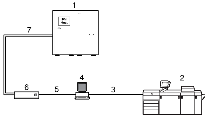
Figure 1-1. Printing system: channel-attached configuration
