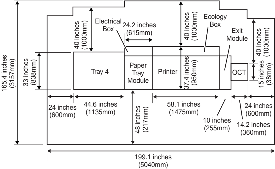
Figure 6-5. Printer with Tray 4
