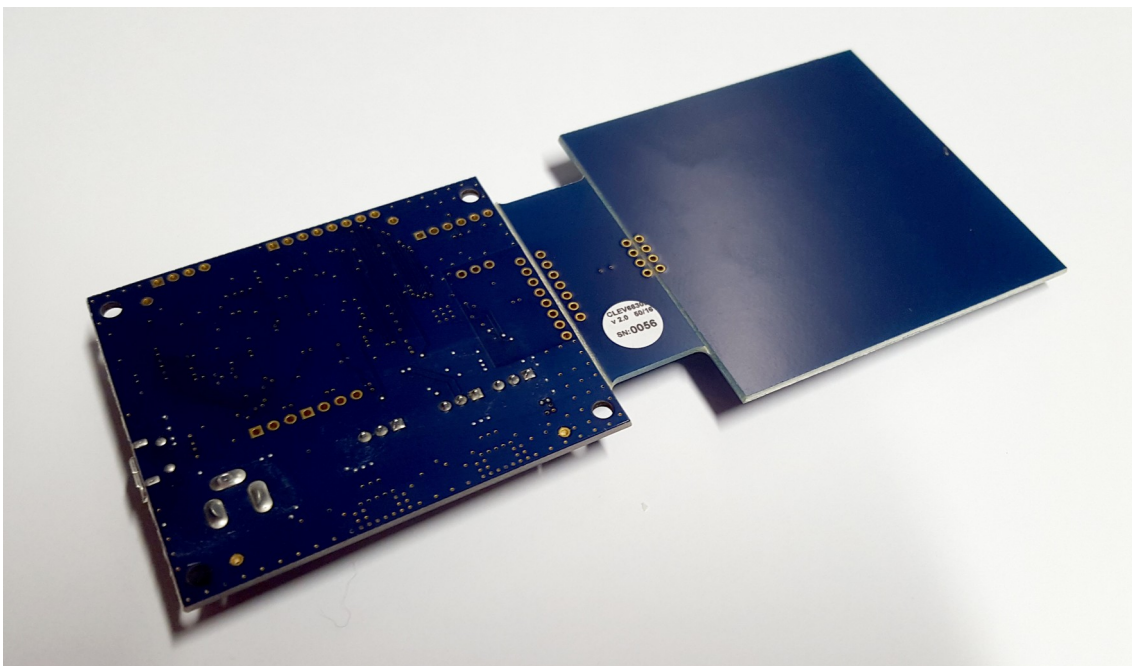
Figure 2: Customer Evaluation Board CLRC663, CLEV6630B – bottom view.
