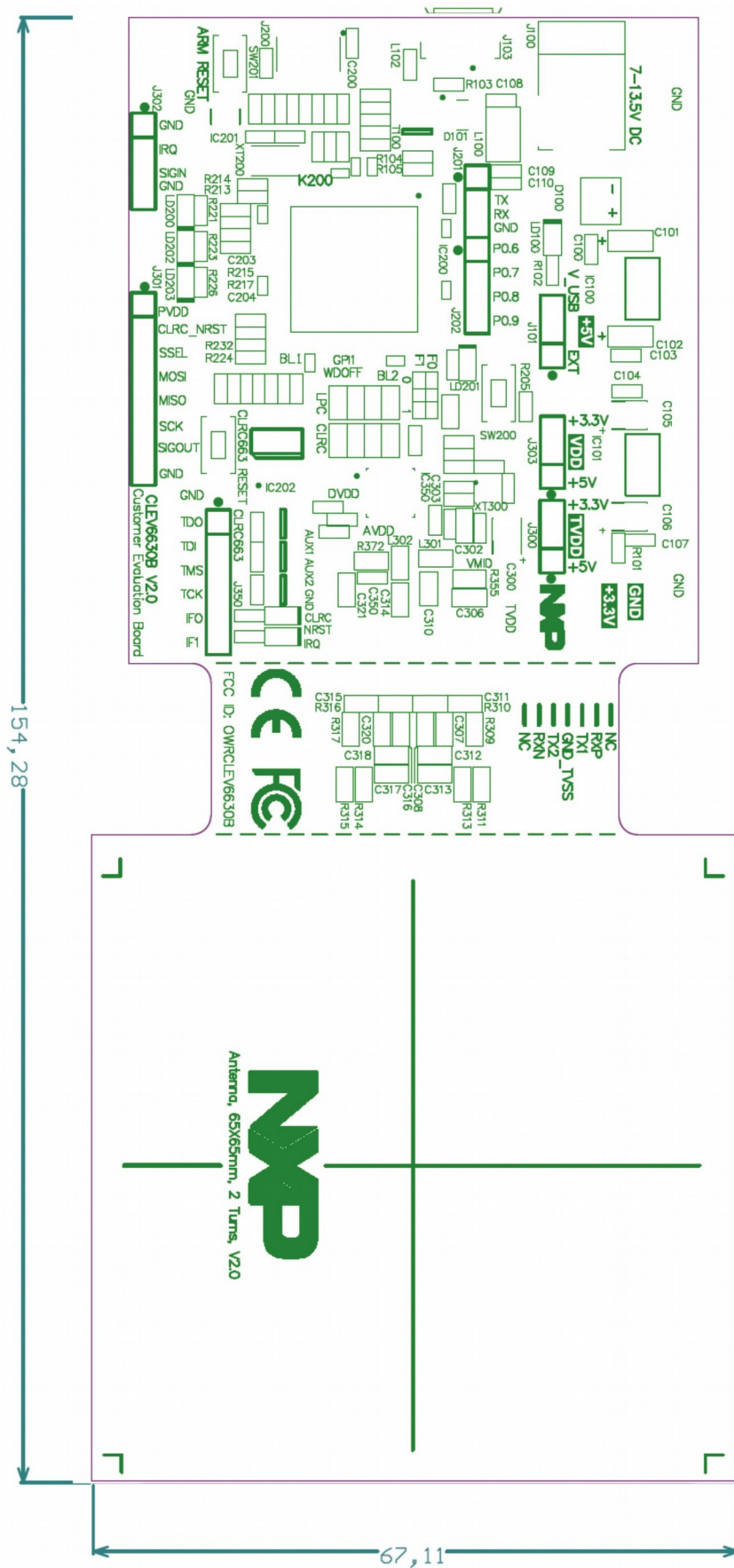
Figure 4: Customer Evaluation Board CLRC663, CLEV6630B: dimensions, pcb with elements.
