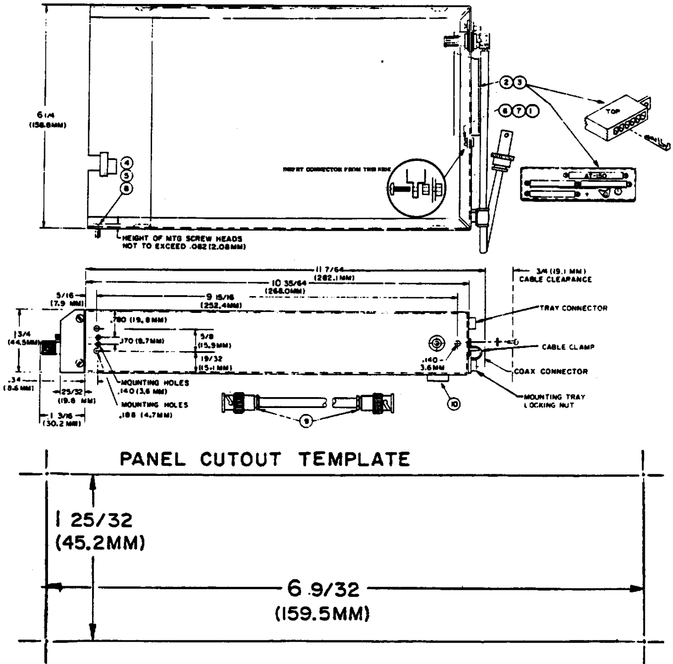
FIGURE 2-2. INSTALLATION DIAGRAM
