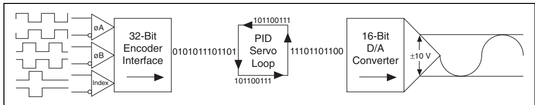
Figure 4-1. Servo Axis Resources
