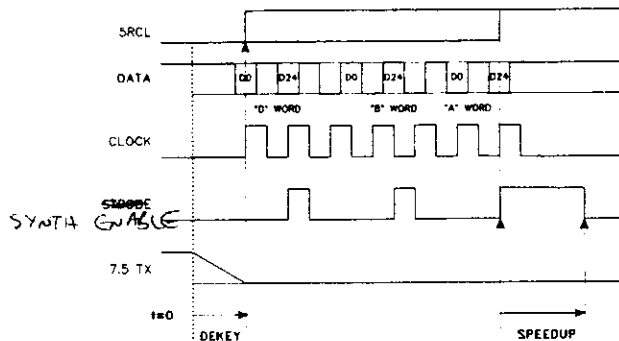
Figure 3-6 TX TO RX TIMING DIAGRAM
