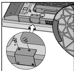
Main switch cover (with stand) The longer side of the cover is toward the bottom of the display.
