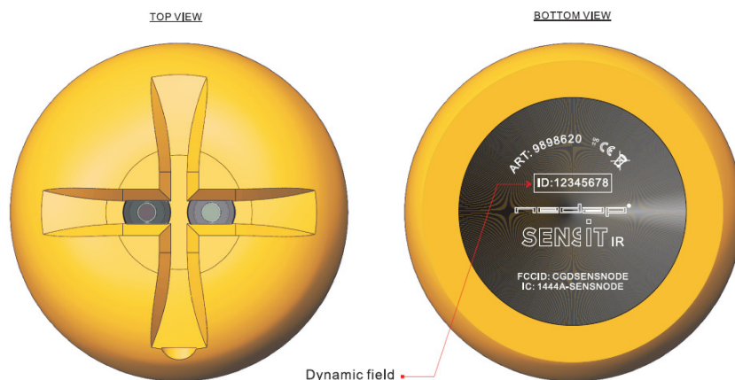
Figure 2: Top and bottom laser engraved side of the SENSIT IR
