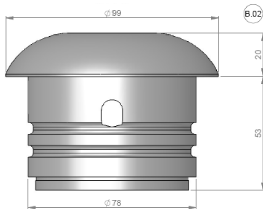
Figure 1: Dimensions SENSIT IR
