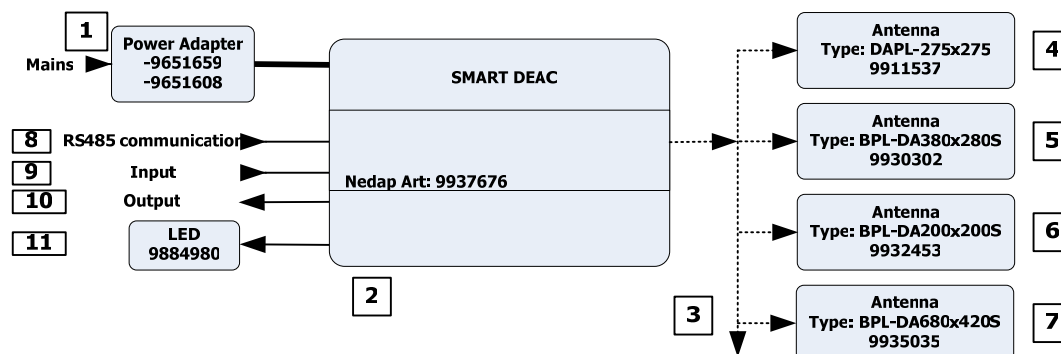
Figure 1 Functional system overview
