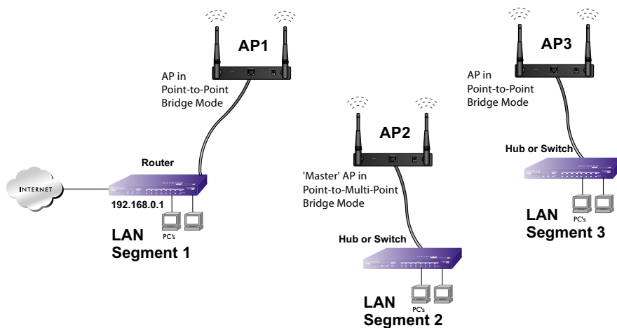
Figure 5-7 Wireless point-to-multipoint bridge setup
