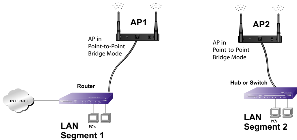
Figure 5-6 Wireless point-to-point bridge setup
